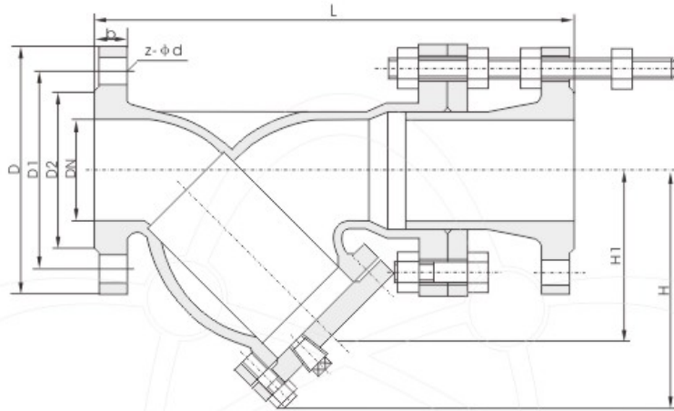
主要外形和连接尺寸 Main external and connecting dimensions
